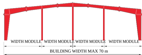
Hitech Multi Gable (HMG)
