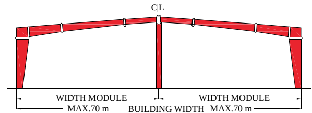
Hitech Multi Span (HMS-3)
