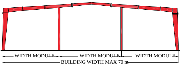
Hitech Roof System (HRS)
